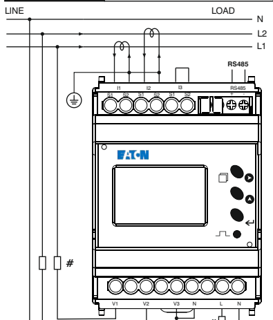
2 Phase - 3 Wire 2 Ø - 3 Wire, 2 CT'S
