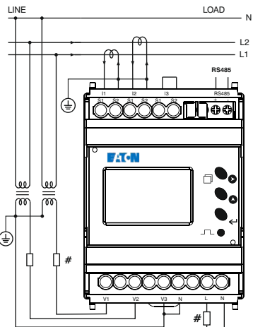
2 Phase - 3 Wire 2 Ø - 3 Wire, 2 CT'S and 2 PT'S
