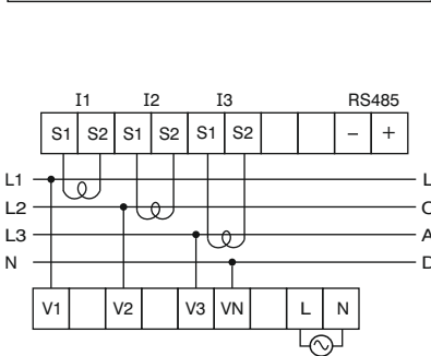
TERMINAL CONNECTIONS
