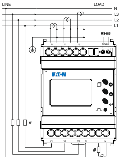
3 Phase-4 Wire (Commonly Used) 3 Ø - 4 Wire, 3 CT'S
