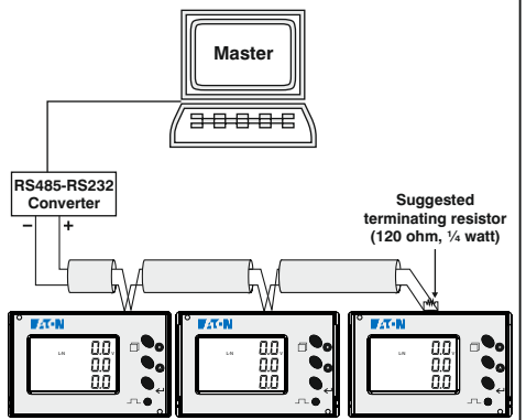
CONNECTION DIAGRAM FOR COMMUNICATION
