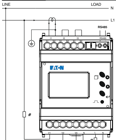
1 Phase - 2 Wire 1 Ø - 2 Wire, 1 CT
