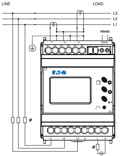
3 Phase - 3 Wire 3 Ø - 3 Wire, 2 CT'S
