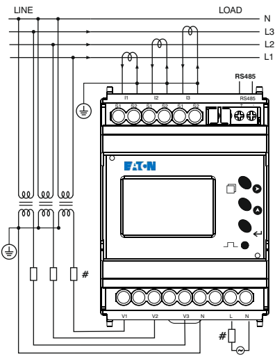
3 Phase - 4 Wire 3 Ø - 4 Wire, 3 CT'S and 3 PT'S
