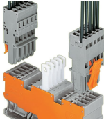
2-pin disconnect carrier terminal block with two jumper positions 1-conductor female plug, straight* *1-conductor angled female plug is also possible!
