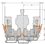
Carrier terminal block For other dimensions, see carrier terminal block (769-151).
