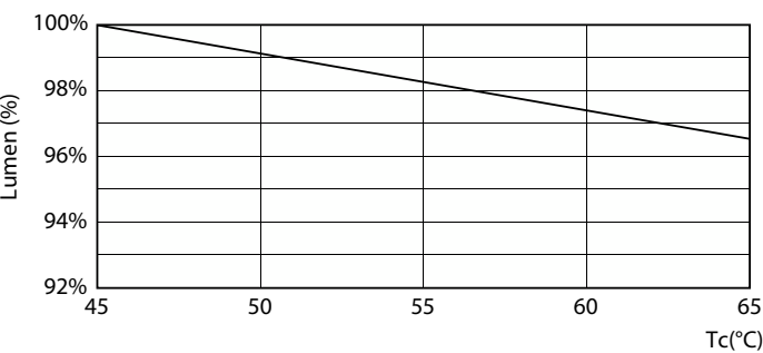
Lumen Maintenance Diagram - CorePro LEDtube HF 1200mm HO 26.7W 865T5
