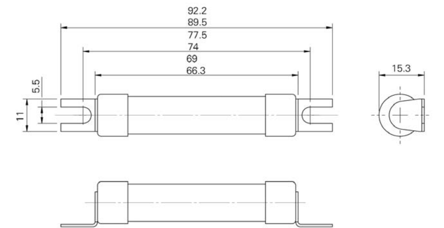
Cylindrical with Tags PV-(amp rating)A14L-T
