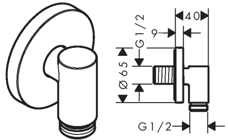
FixFit Fine S 28882XX0 / 28882XX7
