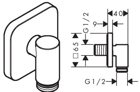
FixFit Fine Q 28884XX0 / 28884XX7
