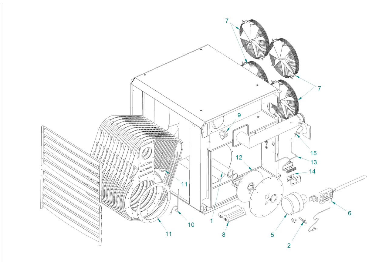
Figuur 24 - Exploded view van de XR10+ - XR120+
