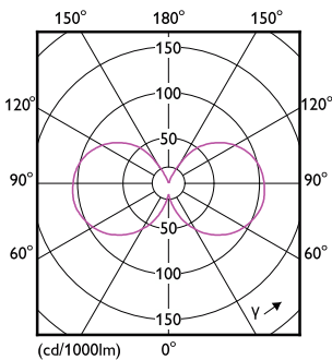
Light Distribution Diagram - CorePro LEDBulbND 7-60W E27 A60 830 FR G
