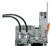
1-conductor female plug Carrier terminal blocks can be commoned via 280 and 780 Series Jumpers and tested using a test plug adapter (280-4..).
