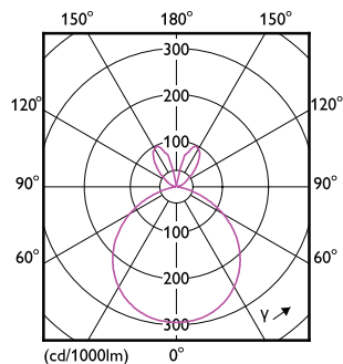
Light Distribution Diagram - CorePro LEDlinearND 11.5-100W R7S78mm830
