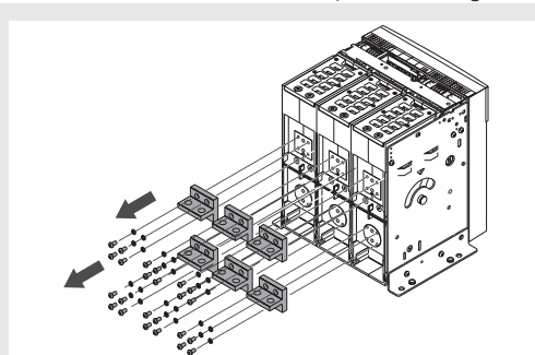
Figure 65 IEC
