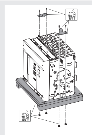
Figure 11 Partie mobile IEC
