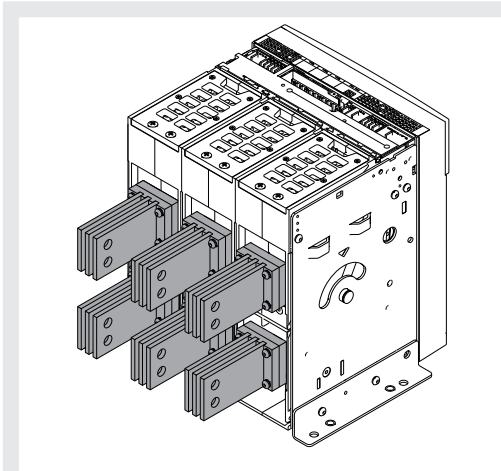
Figure 63 VR - Arrière verticales UL Listed
