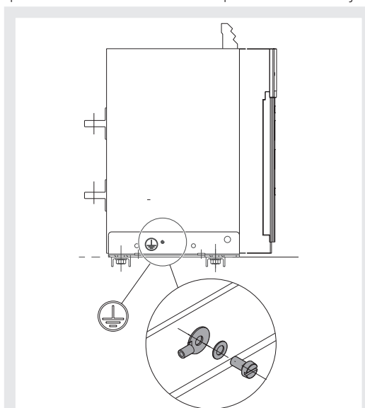
Figure 73 - Version fixe
