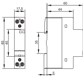
CR20
