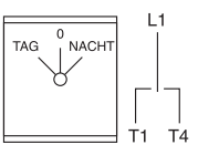
Z-DSU1-T0N
