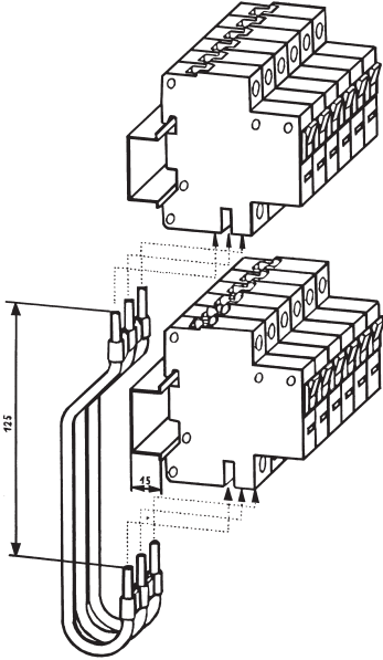
RVS-3PHAS/125
