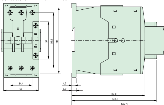
Contactors DILM40-DILM65
