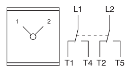
Z-DSU2-12
