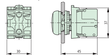
Installation depth
