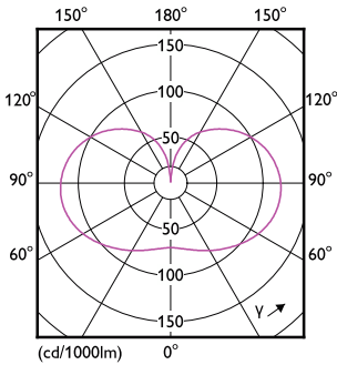
Light Distribution Diagram - CorePro LEDBulbND 200W E27 A95 865 FR G
