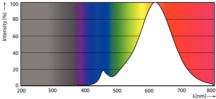
Spectral Power Distribution Colour - CorePro LEDBulbND 7-60W E27 ST64 827CL G
