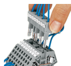
B-type test plug modules fitted with CAGE CLAMP®
