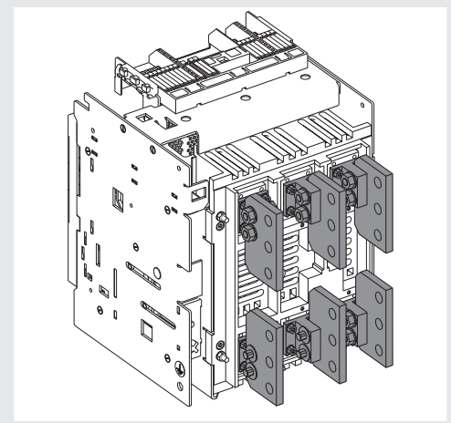
Abbildung 57 - F - FC - Kabelanschlüsse IEC-UL
