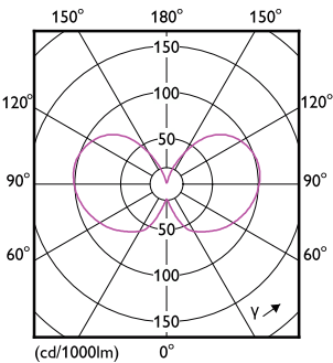
Light Distribution Diagram - MAS LEDBulbND2.3-40W E27 840 A60 FR G UE
