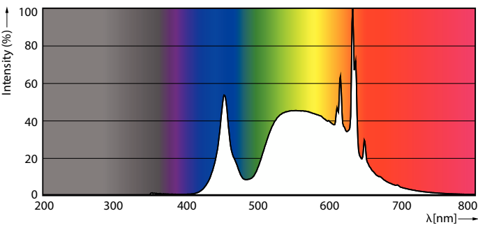
Spectral Power Distribution Colour - MAS LEDBulbND2.3-40W E27 840 A60 FR G UE
