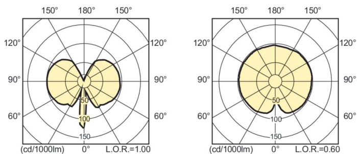
Light Distribution Diagram - MC CDM-Tm Elite Mini 20W/830 GU6.5 ICT
