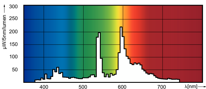
Spectral Power Distribution Colour - MC CDM-Tm Elite Mini 20W/830 GU6.5 ICT
