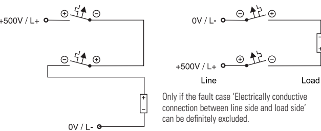
Connection example at 500 V=, 2-pole
