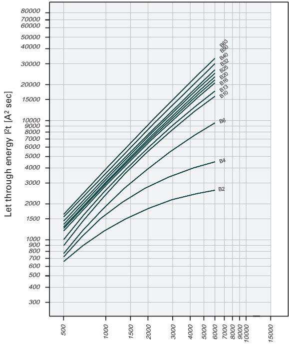
Let-through Energy PL6, Characteristic B, 1-pole
