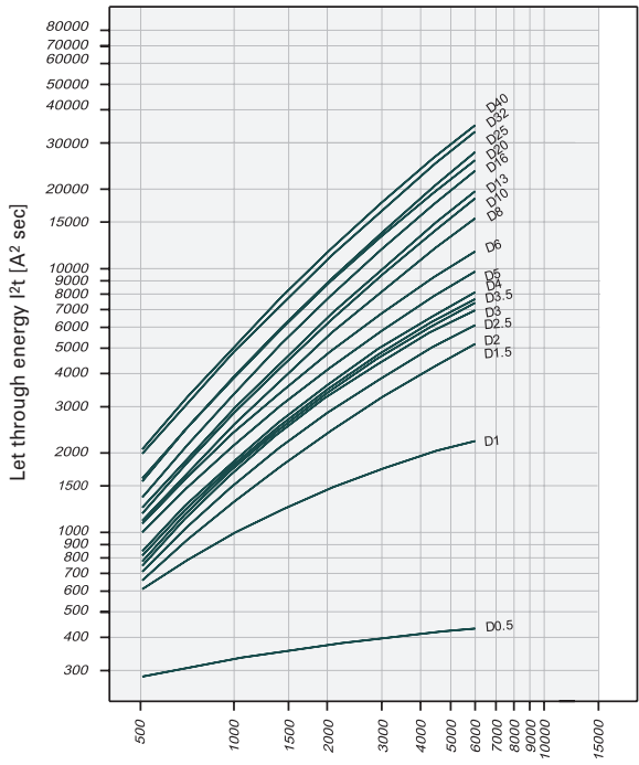
Let-through Energy PL6, Characteristic D, 1-pole
