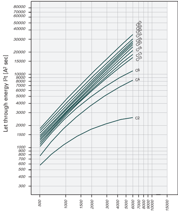
Let-through Energy PL6, Characteristic C, 1-pole
