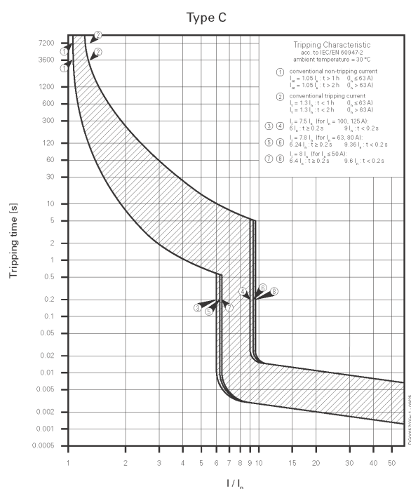
Time-Current Characteristics, Type C
