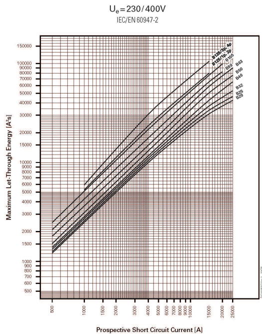
Maximum Let-Through Energy, Type B
