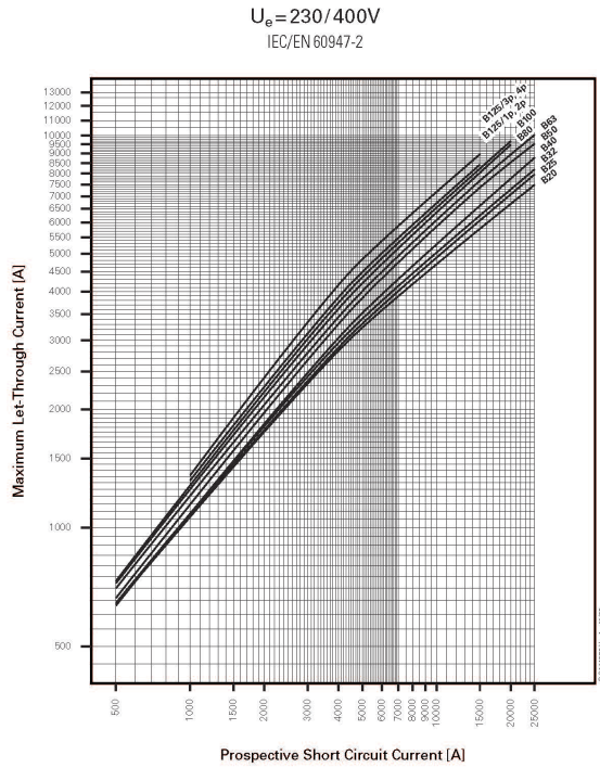
Maximum Let-Through Current, Type B
