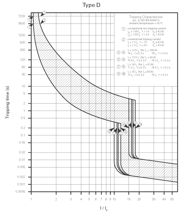
Time-Current Characteristics, Type D
