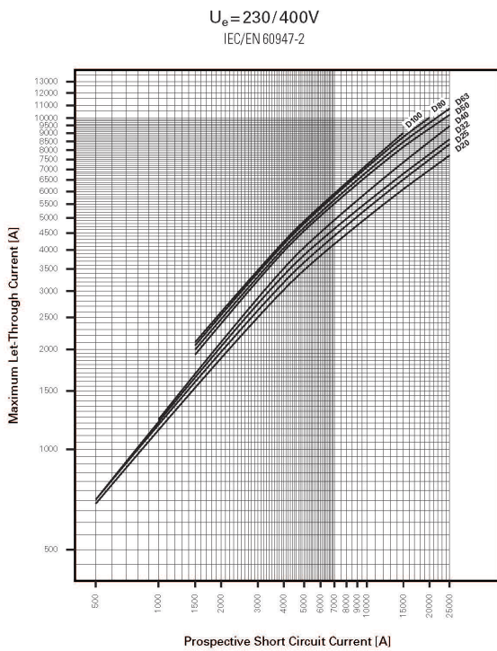
Maximum Let-Through Energy, Type D
