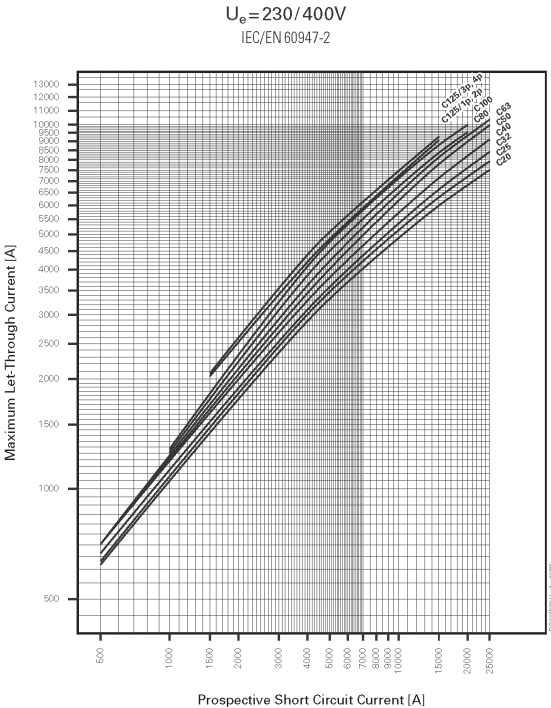
Maximum Let-Through Current, Type C
