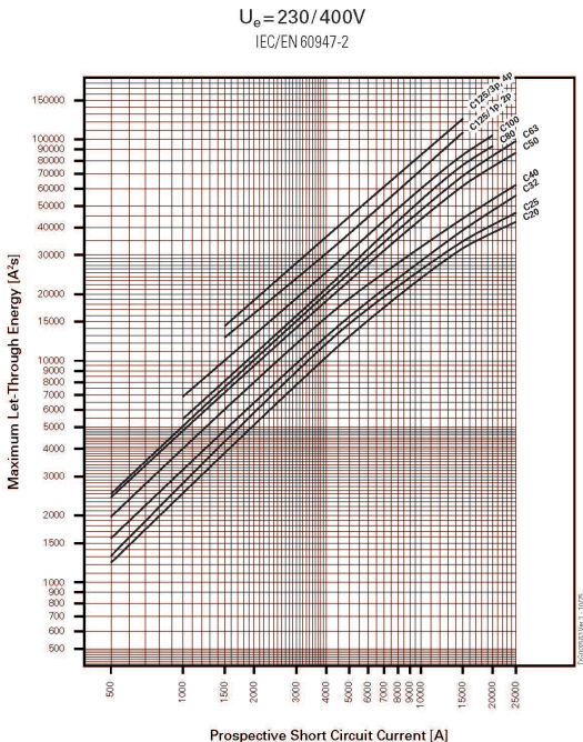
Maximum Let-Through Energy, Type C
