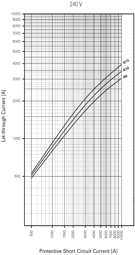
Let-through Current FRBdM, Characteristic B
