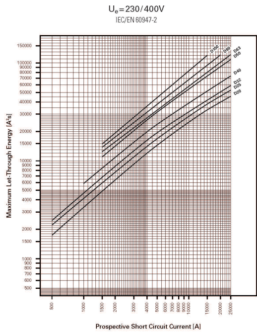
Maximum Let-Through Energy, Type D
