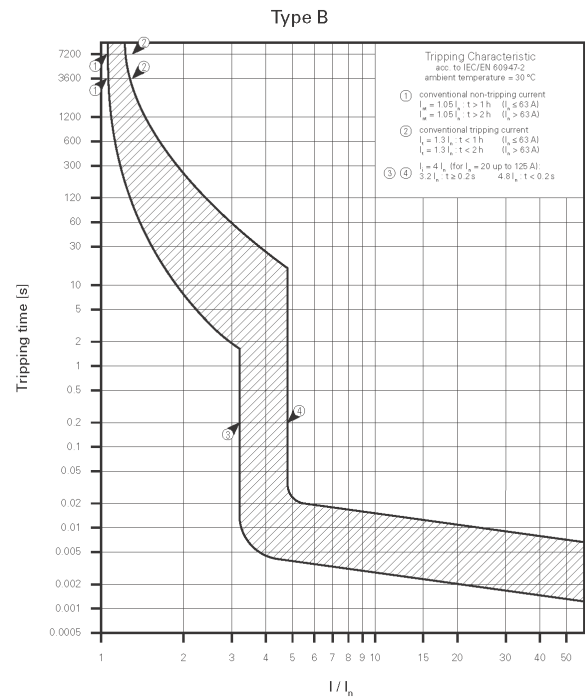
Time-Current Characteristics, Type B
