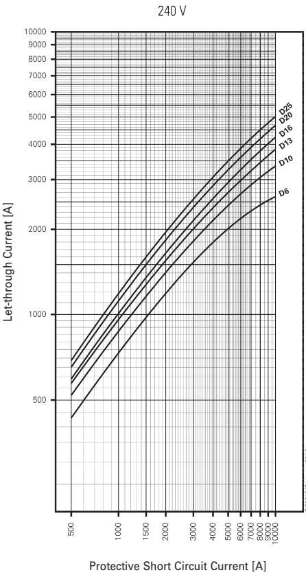
Let-through Current FRBdM, Characteristic D
