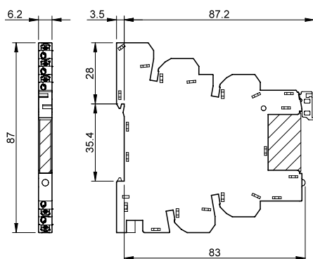
Type 39.01.0.024.0060 1 wisselcontact 6 A 250 V AC1
