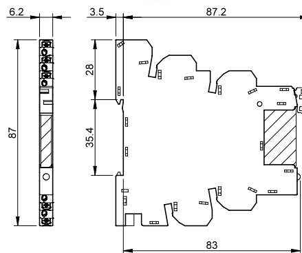
Type 39.01.0.024.xx73 1 wisselcontact 6 A 250 V AC1
