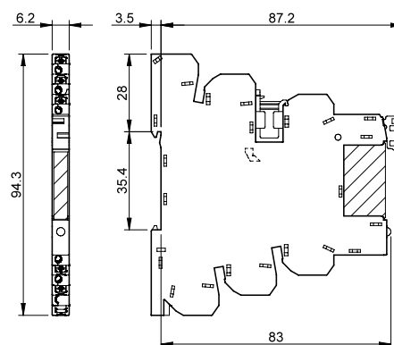
Type 39.61.7.024.0060 1 wisselcontact 6 A 250 V AC1
