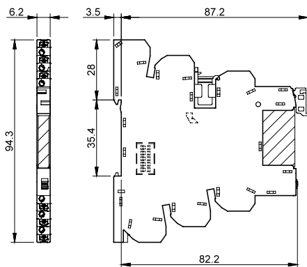
Type 39.90.0.024.9024 1 maakcontact 6 A 24 V DC
