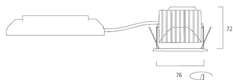
Dimensions (mm)
