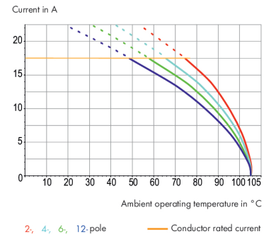
Current-Carrying Capacity Curve Pin spacing: 3.96 mm / Conductor cross-section: 1.5 mm 2 "e" Based on: EN 60512-5-2 / Reduction factor: 1
