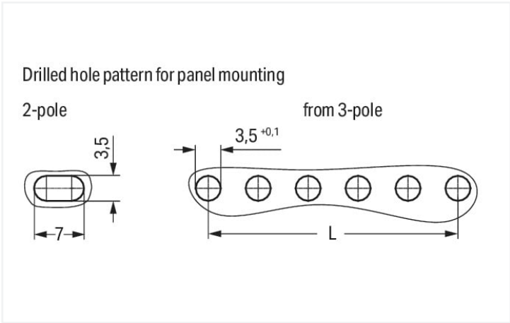
Dimensions in mm Even pole number: L = (pole no. – 2) x pin spacing Odd pole number: L = (pole no. – 1) x pin spacing
