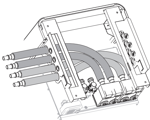
CONFIGURATIE 3 | Cv links + Bron links
