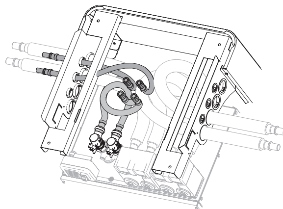
CONFIGURATIE 6 | Tapwater links + Cv links + Bron rechts
