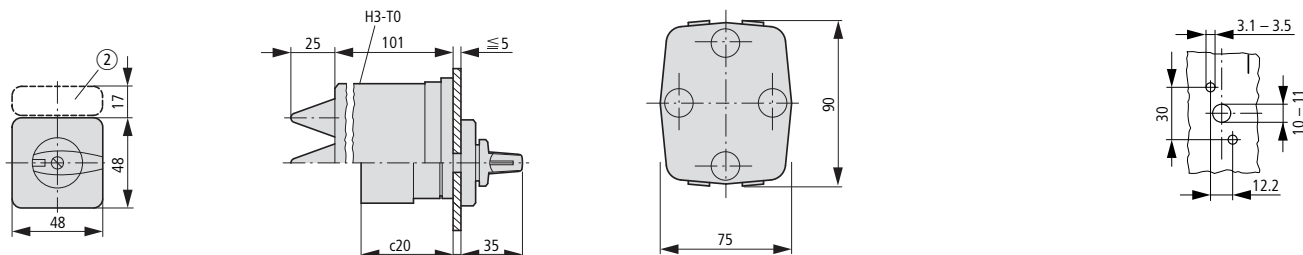
Drilling dimensions
