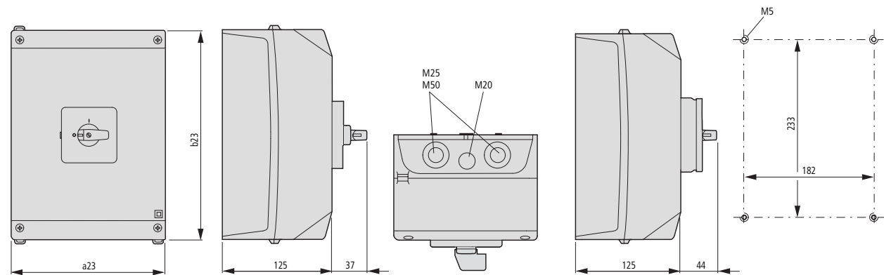
Drilling dimensions
