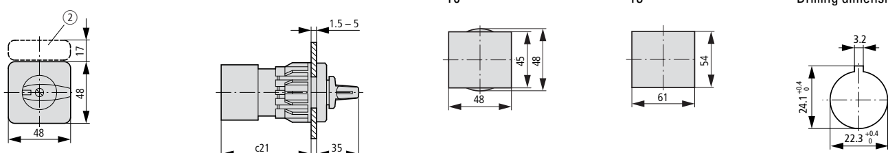
Drilling dimensions
