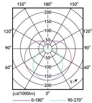
Light Distribution Diagram - MAS LEDtube Mains/EL 1500mm 26W 840 T5
