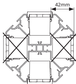
ALK54../.. ALK5400/..
