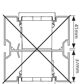
ALK22../.. ALK2200/..
