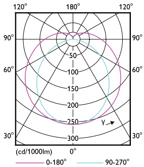
Light Distribution Diagram - MAS LEDtube Mains/EL 600mm 7.6W 840 T8
