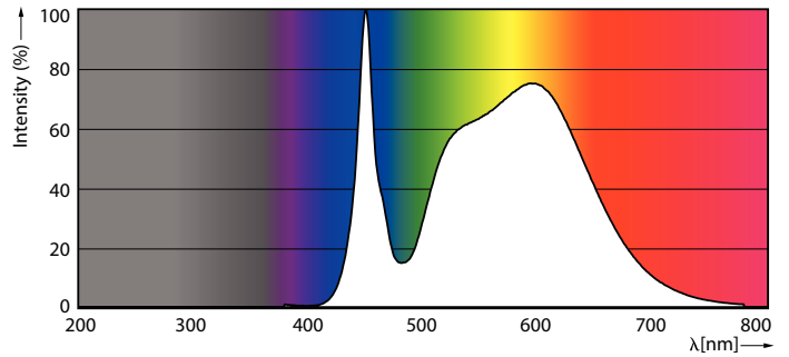
Spectral Power Distribution Colour - MAS LEDtube Mains/EL 600mm 7.6W 840 T8
