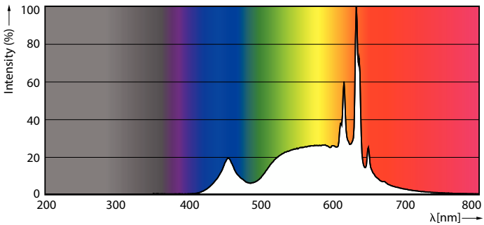
Spectral Power Distribution Colour - CorePro LEDbulb ND 4.9-40W A60 E27 930
