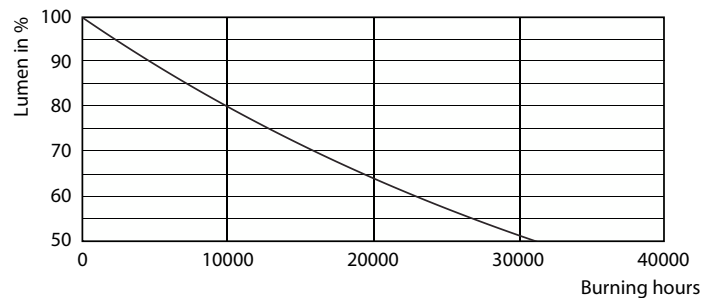
Lumen Maintenance Diagram - CorePro LEDBulbND 7-60W E27 A60 827FR
