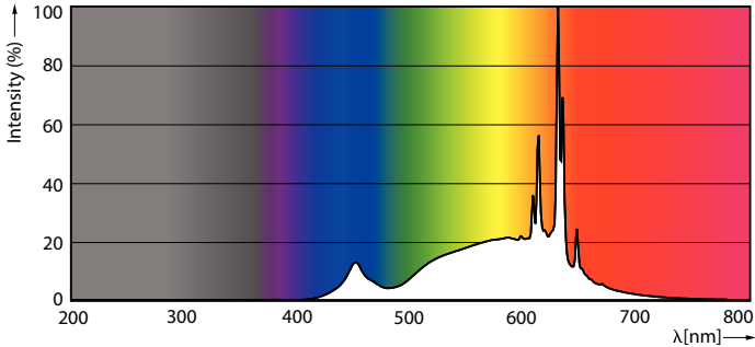
Spectral Power Distribution Colour - MAS LED spot VLE D 5.5-80W GU10 927 36D
