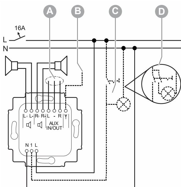
Fig. 8: Electrical connection
