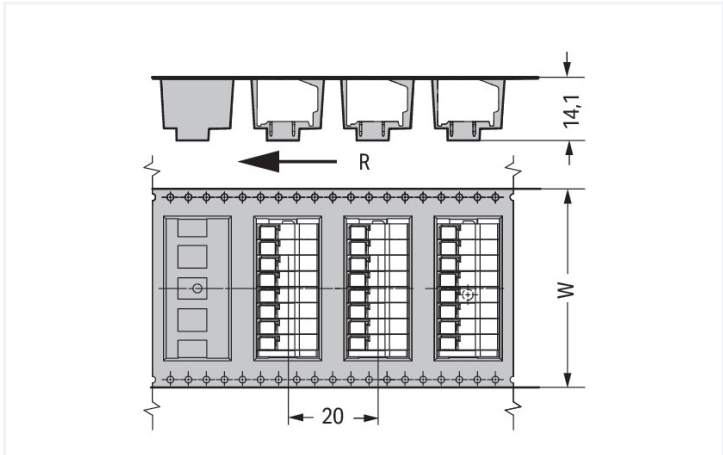
Dimensions in mm R = feed direction W = tape width
