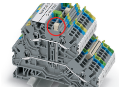
Commoning two levels via double-deck vertical jumper (Item No. 2000-492).
