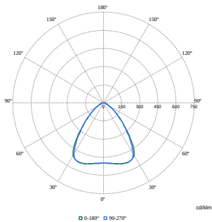
Polar Normal (separate) - RC340BI - 910925867039
