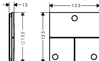
AXOR ShowerSelect ID square 36780XX0 / 36815140
