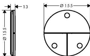
AXOR ShowerSelect ID round 36779XX0 / 36814140
