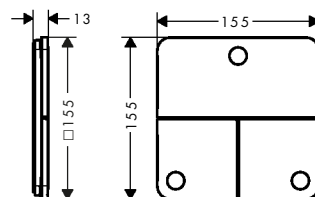
AXOR ShowerSelect ID softsquare 36781XX0 / 36816140
