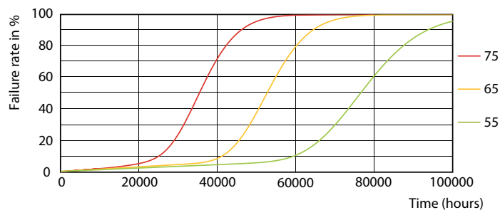
LEDtube-75K-5575-FailureRate-LED
