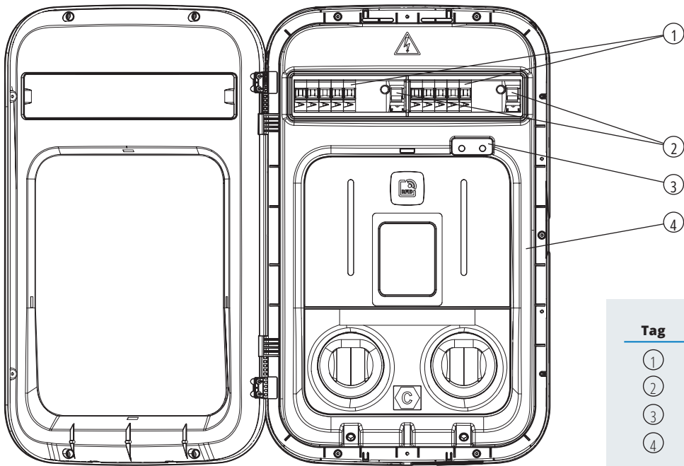
Figure 5. Green Motion Duo safety switchgear components and buttons
