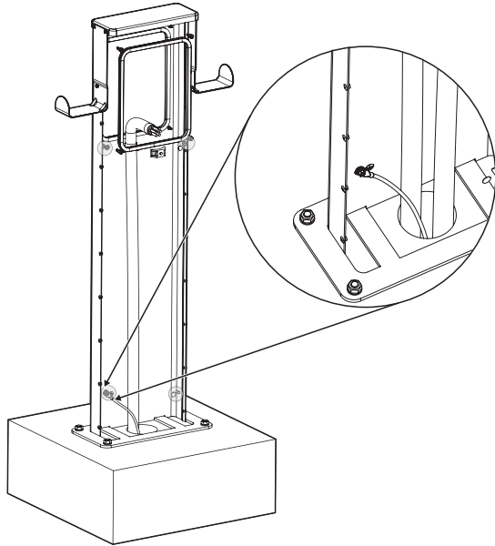
Figure 25. Grounding studs location.
