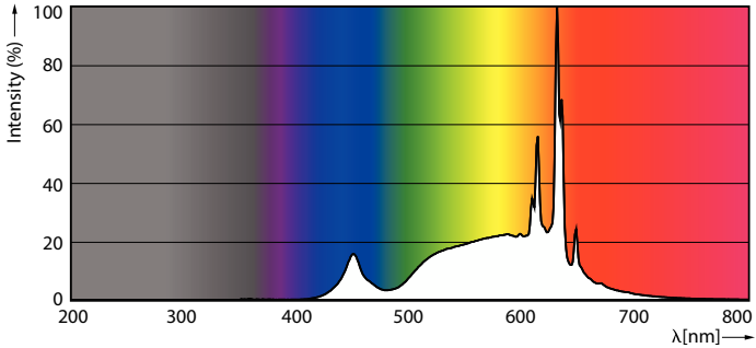
Spectral Power Distribution Colour - MAS LEDCandleDT2.5-25W E14 BA35 CL G
