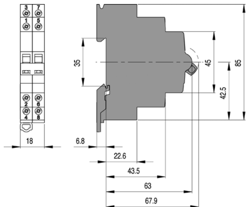
Switch, 3+4-pole
