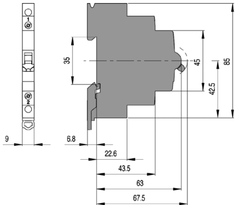
Switch, 1+2-pole
