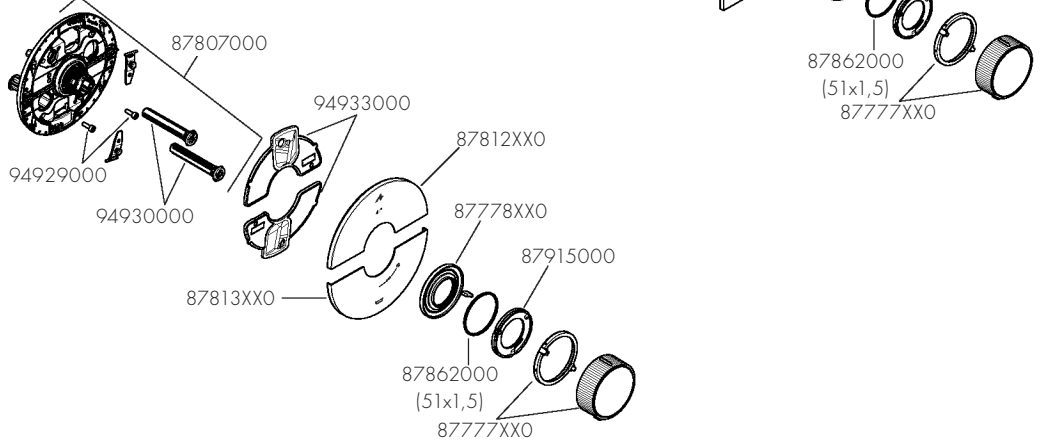
AXOR ShowerSelect ID round 36751XX0
