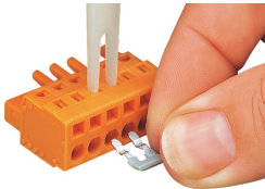
Operating tool for comb-style jumper bars (231-902)
