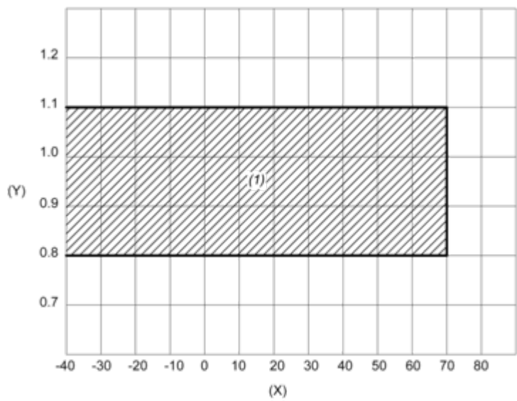
AC Coil Operating Range VS Ambient Temperature
