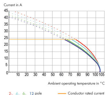
Current-Carrying Capacity Curve Pin spacing: 5 mm / Conductor cross-section: 2.5 mm 2 "I st " Based on: EN 60512-5-2 / Reduction factor: 1
