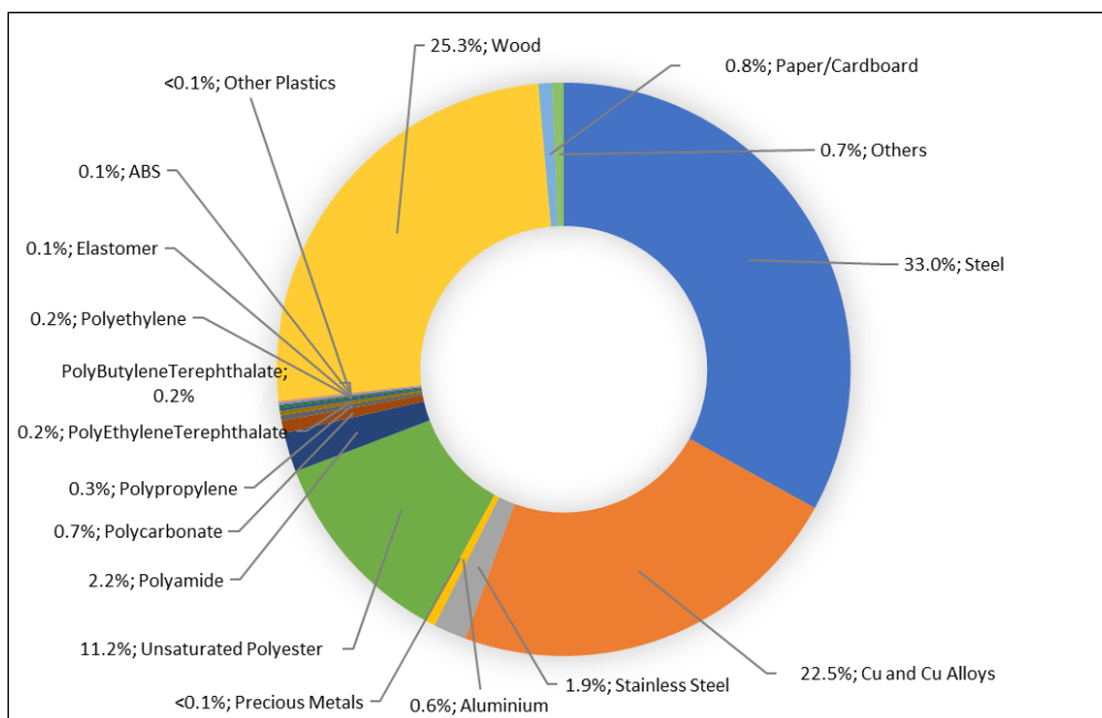
Figure 1: Composition of E2.2 N 2500A 3P
