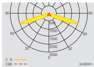
i-P65 E CG-S with asymmetric optics
