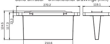
Cone diffuser - Dimensional drawings (mm)
