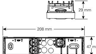
Add-on housing
