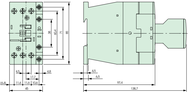
Contactors DILM17-DILM32
