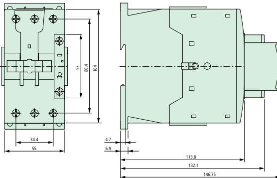
Contactors DILM40-DILM65
