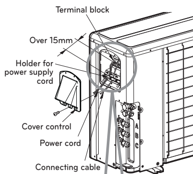
Loosen terminal screw
