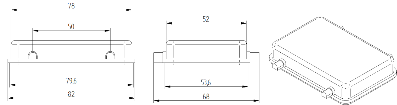
EPIC® H-A 32 KDB (without safety cord), 10481700
