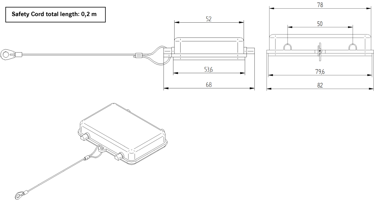
EPIC® H-A 32 KDBF (with safety cord), 10481500
